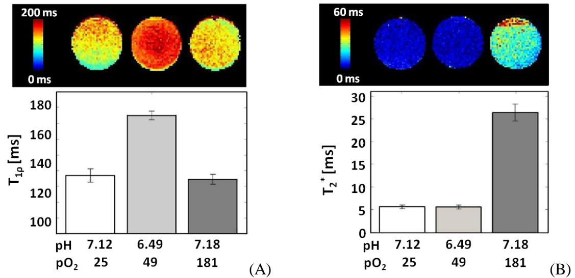
Figure 3.2. T_{1\rho} measurements of sheep blood phantoms across a pH and oxygenated spectrum. (A) T_{1\rho} maps and measurements of sheep blood phantoms in control (left), acidified (center), and oxygenated (right) conditions demonstrating T_{1\rho} increases with a decrease in blood pH and is independent of the oxygenated state of hemoglobin. (B) BOLD maps and measurements of sheep blood phantoms in control (left), and acidified (center), and oxygenated (right) conditions demonstrating BOLD is dependent of the oxygenated state of hemoglobin and independent of the pH of the blood.
