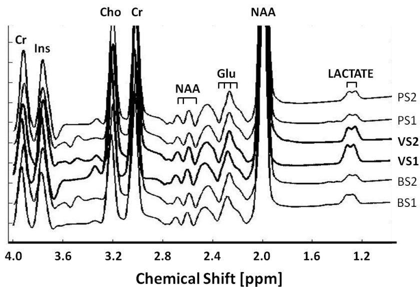
Figure 4.1. Localized 1 H MR spectra for baseline, visual stimulation, and post-stimulus. The six spectra shown were obtained consecutively from the same voxel in the same subject. Stack plot of spectra obtained before (baseline 1, BS1 and baseline 2, BS2), during (visual stimulation 1, VS1 and visual stimulation 2, VS2), and following visual stimulation (post-stimulus 1, PS1 and post-stimulus 2, PS2). In vivo metabolites include N-acetylaspartate (NAA), creatine (Cr+PCr), choline (Cho), myo-inositol(Ins), and glutamate (Glu).
