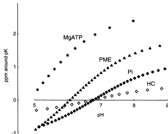
Figure 2.18. Titration curve of three signals (MgATP, PME and Pi) in the ^{31}\text{P} MRS and homocarnosine (HC) in the ^1\text{H} MRS [14].
