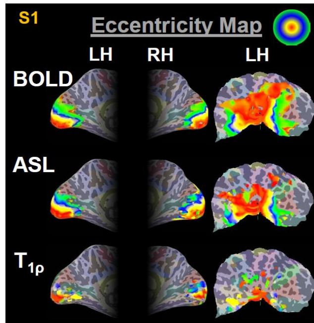
Figure 6.1. Eccentricity maps of BOLD, ASL, and T_{1\rho} response to the expanding ring stimulus on the left and right inflated hemisphere, and the left flattened brain surface for single subject (S1). The color scale indicates the raw phase value between 0 and 2\pi for eccentricity map. The red color indicates regions corresponding to the center of field of view, while the green color regions correspond to the outer eccentric degrees.
